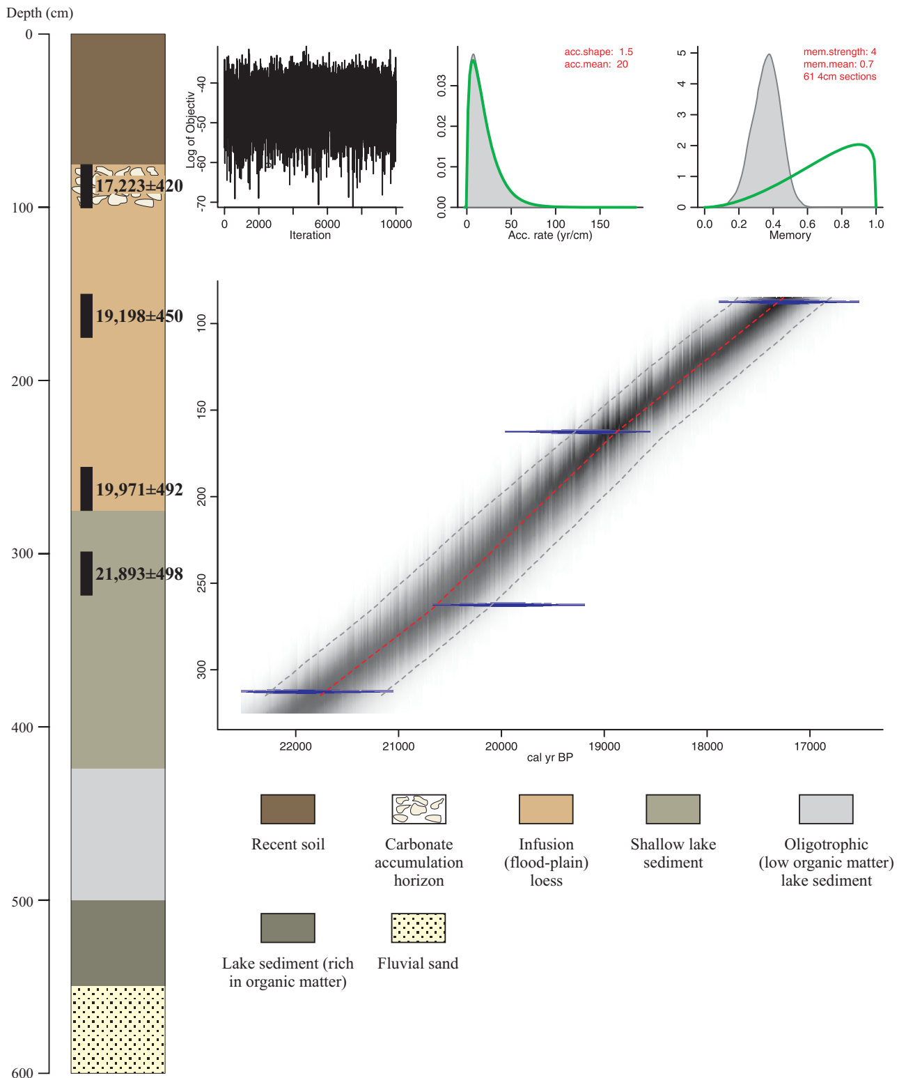
Fig. 4. Lithology of the infusion loess (Profile #2) profile and the constructed age-depth model.
